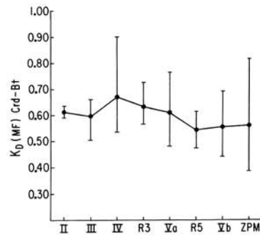
Fig. 4. Variation with grade of K_D = (Mg/Fe)_{Bt}/(Mg/Fe)_{Crd} . The heavy dots are the mean of the values from each zone, with the brackets indicating the range. Numerical data are listed in Table 3.
