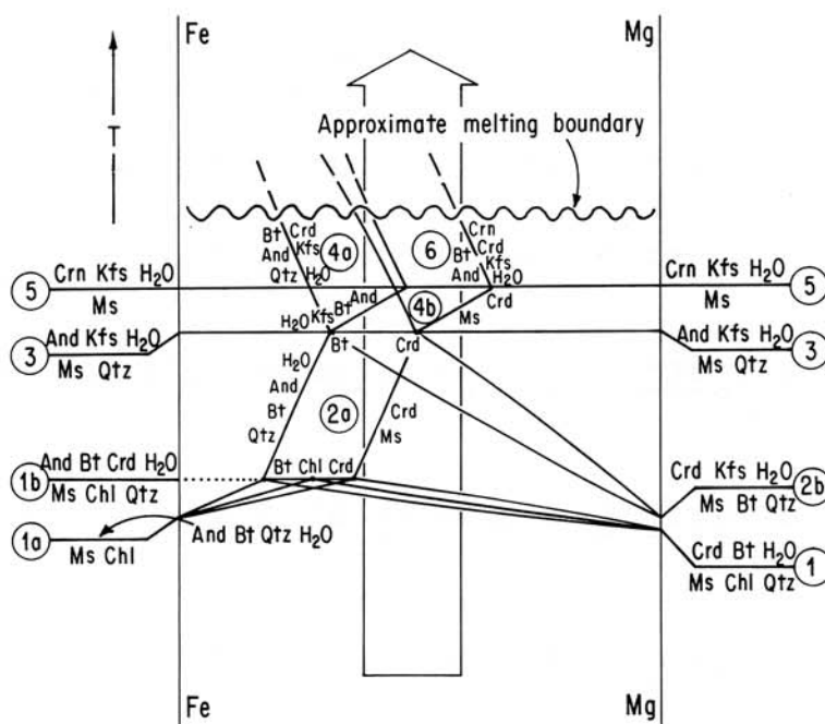
Fig. 2. Schematic isobaric T-X_{\text{Fe-Mg}} diagram for the divariant reactions in the Ballachulish aureole (see Table 1 for the correspondence of the thermal aureole zones with the reactions). The broad arrow encompasses the bulk of the \text{Mg}/(\text{Mg} + \text{Fe}) compositional variation of the pelites in the aureole.
