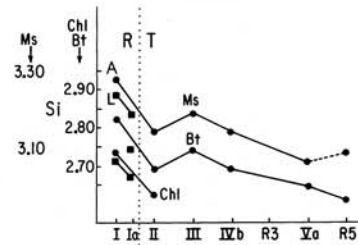
Fig. 8. Comparison of the variation with grade of Si in muscovite, biotite, and chlorite in the Appin Phyllite (contact metamorphism = heavy dots) and the Leven Schist (regional metamorphism = squares). The symbols are the same as used in Figs. 5-7.
