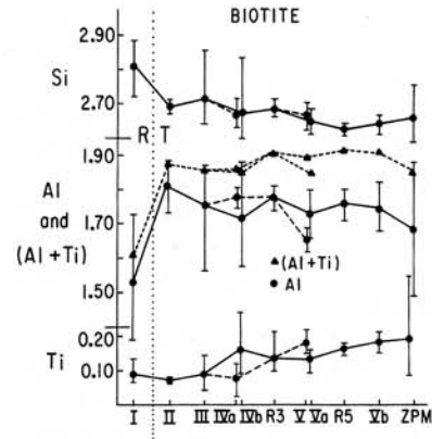
Fig. 7. Variation with grade of Si, Al, Ti, and Al + Ti in biotite from all units. ZPM = Zone of partial melting; all other symbols the same as in Figs. 5 and 6. The lines joining zones IVa and V to the overall trend have been dashed to distinguish them from zones IVb and Va, which occur at the same grade. Numerical data are listed in Table 3.
