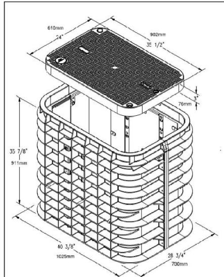
CHANNEL 24x36x36 ENCLOSURE DETAIL N.T.S.
