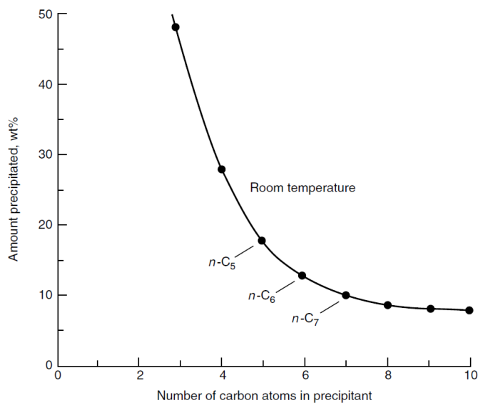
Figure 2.4 Change in asphaltene yield with carbon number of paraffin used (Adapted from Speight, 2007).
