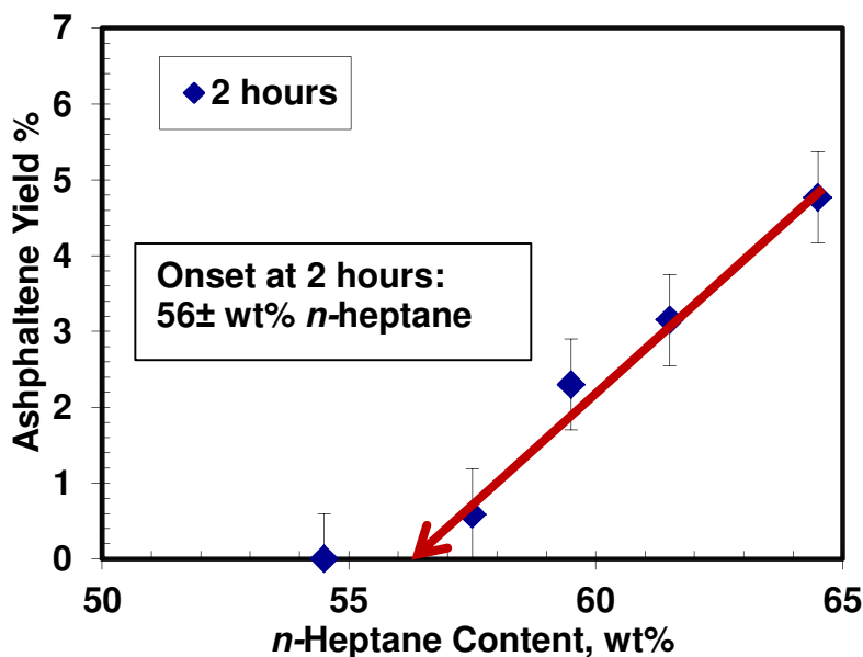
Figure 4.2: Gravimetric determination of the onset of asphaltene precipitation from n -heptane diluted WC_B2 bitumen at 2 hours by extrapolation of asphaltene yield data to zero yield at 23°C.
