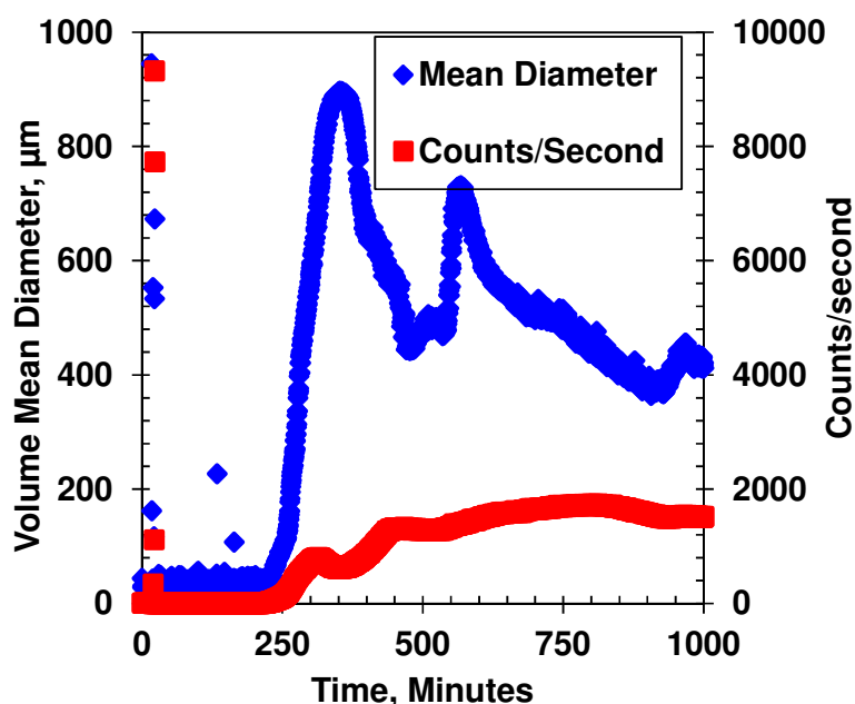
Figure 6.7: Volume mean diameter and particle count measurements at longer time for 61.5 wt% n -heptane, using two-stage mixing method at 195 rpm, and 23°C.
