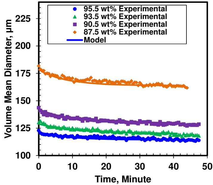
Figure 6.20: Case 1 model fitted to data for 87.5-95.5 wt% n -heptane diluted bitumen using the two-stage mixing method and a mixing speed of 195 rpm at 23°C.
