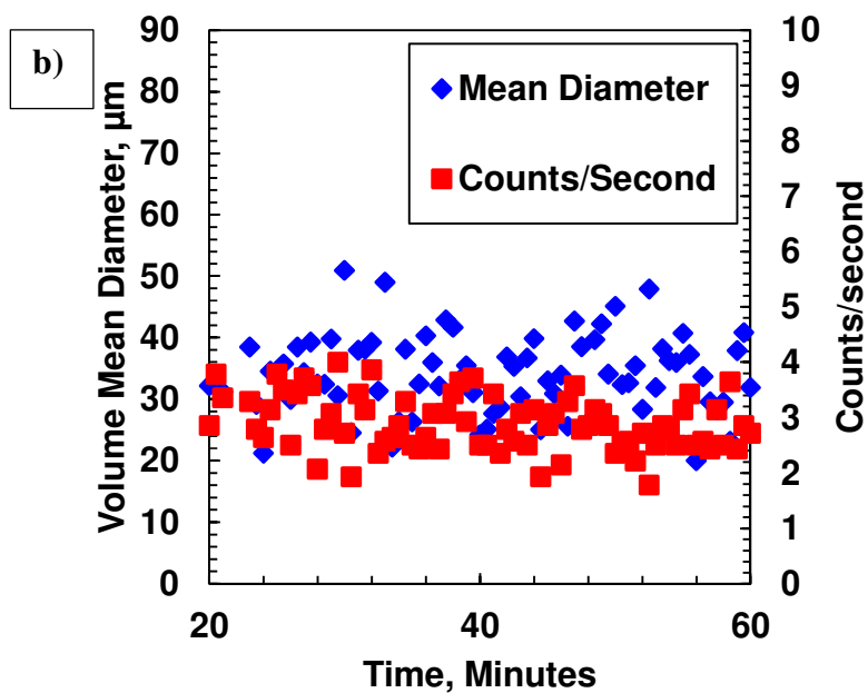
Figure 6.3: Kinetics of asphaltene flocculation at low dilutions of a) 61.5 wt% and b) 65 wt% n -heptane using two-stage mixing method at 195 rpm, and 23°C.
