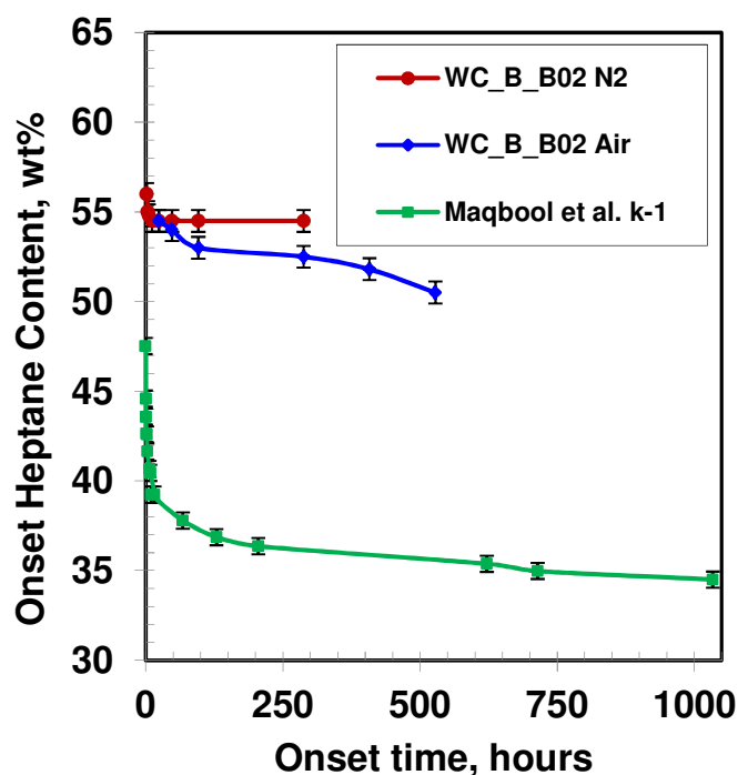
Figure 4.4: Gravimetric precipitation onsets in n -heptane diluted WC_B2 bitumen in air and nitrogen (Shafiee, 2014), and n -heptane diluted k-1 crude oil (Maqbool et al. 2009) at 23°C and 1 atm.
