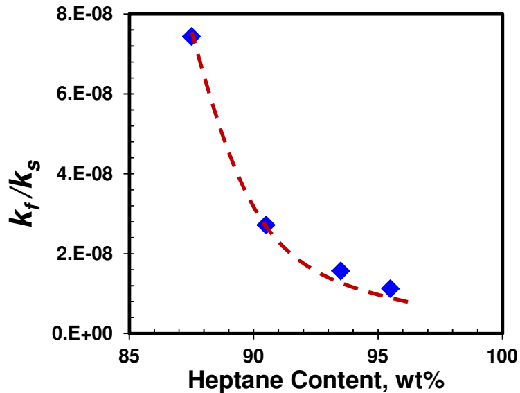
Figure 6.28: The k_f/k_s ratio for the true fractal dimension for 87.5 to 95.5 wt% n -heptane diluted bitumen using the two-stage mixing method and a mixing speed of 195 rpm at 23°C.
