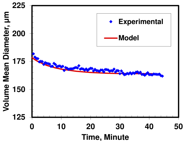
Figure 6.18: The fitted and experimental volume mean diameter for 87.5 wt% n-heptane using two-stage mixing method at 195 rpm, and 23°C.
