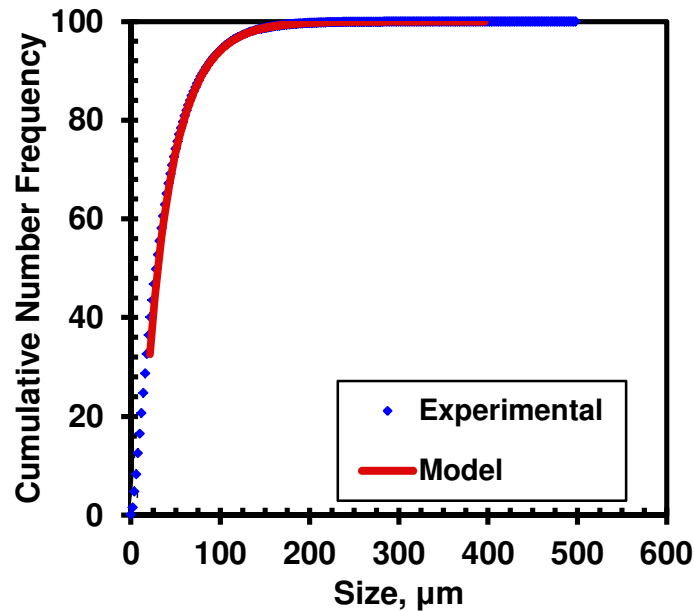
Figure 6.17: Comparison between measured and the converted initial bin cumulative number frequency for 87.5 wt% n-heptane using two-stage mixing method at 195 rpm, and 23°C.
