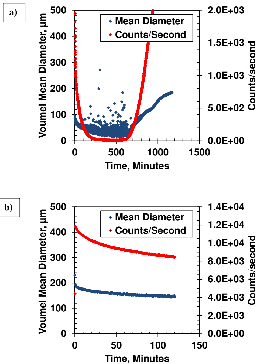
Figure 6.8: Volume mean diameter and particle count measurements at longer time for a) 64.5 wt% n -heptane and b) 70 wt% n -heptane in bitumen diluted with toluene at a 1:1 mass ratio (two-stage mixing method at 195 rpm, and 23°C). Note: the two plots are not on the same scale.
