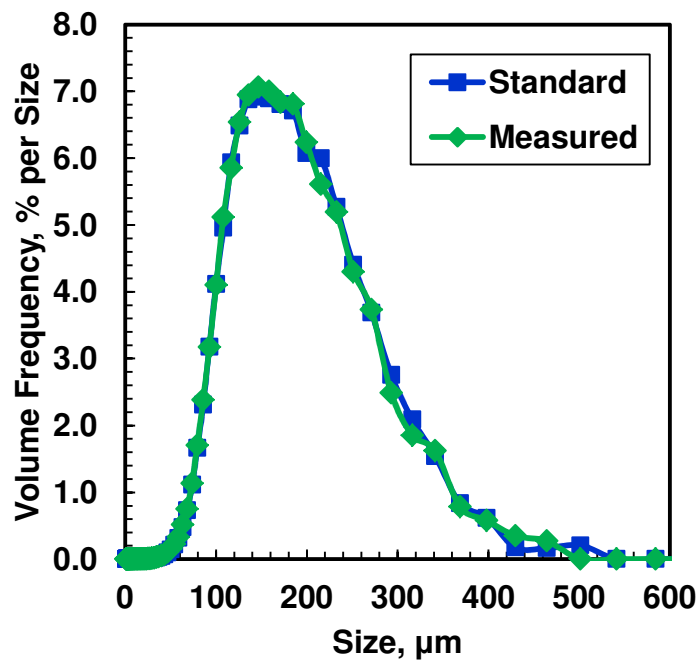
Figure 3.3: Comparison between measured and given volume frequency distribution of a standard sample of 8.33 wt/wt% PVC particles suspended in water at 400 rpm and 23°C.
