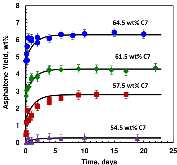
Figure 4.10: Measured and fitted asphaltene yields over time from n -heptane diluted WC_B_B02 bitumen in a nitrogen atmosphere at 23°C and 1 atm.
