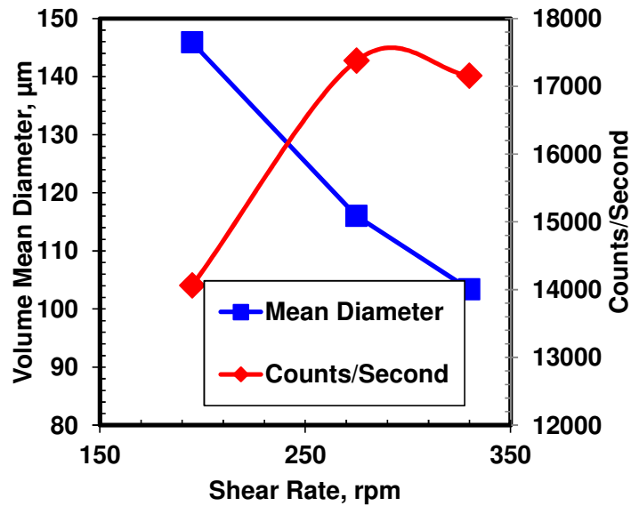
Figure 6.13: Effect of shear rate (mixing rate) on the steady state volume mean diameter and number count rate for 87.5 wt% n -heptane using two-stage mixing scheme at 23°C.
