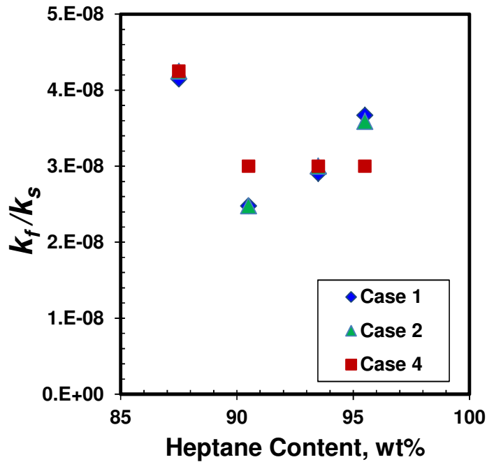
Figure 6.22: The k_f/k_s ratio for each fitting step for 87.5 to 95.5 wt% n -heptane diluted bitumen using the two-stage mixing method and a mixing speed of 195 rpm at 23°C.
