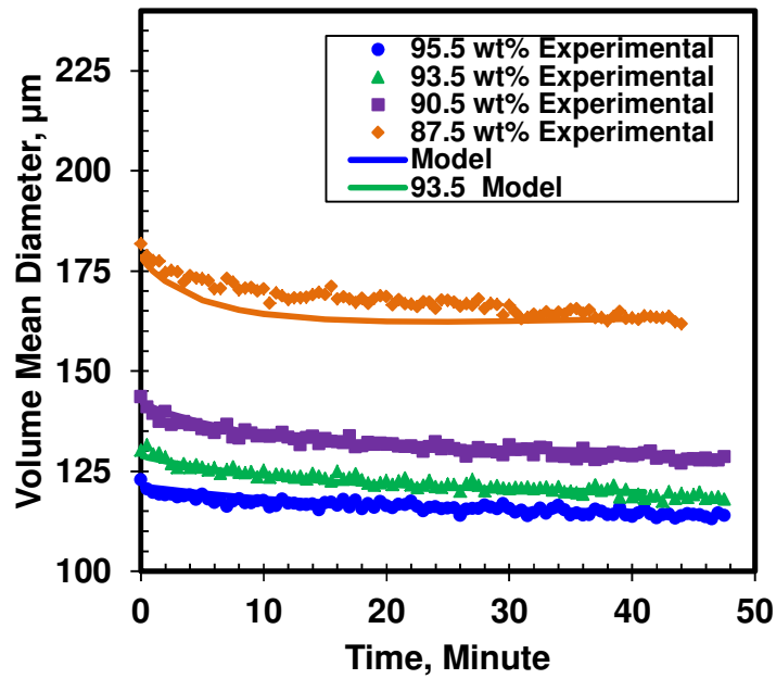
Figure 6.27: Correlated k_f/k_s ratio and constant k_s model results based on true fractal dimension for 87.5 to 95.5 wt% n -heptane diluted bitumen using the two-stage mixing method and mixing speed of 195 rpm at 23°C.
