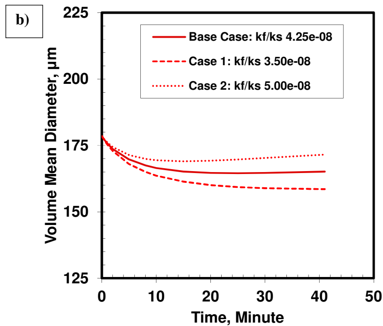
Figure 6.26: Sensitivity of model predictions to k_f/k_s ratios extrapolated to 87.5 wt% n -heptane with different slopes: a) extrapolated k_f/k_s extrapolation; b) predictions for 87.5 wt% n -heptane in W_B02 bitumen using the two-stage mixing method and mixing speed of 195 rpm at 23°C.
