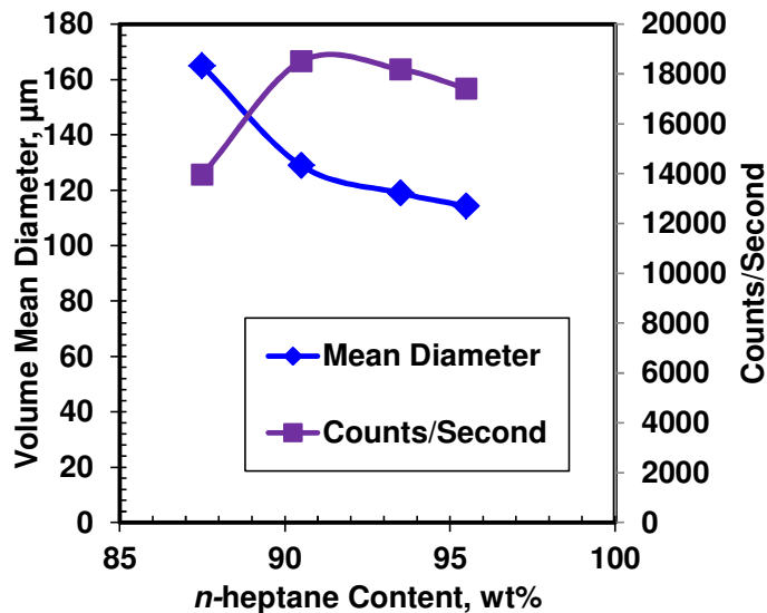
Figure 6.10: Effect of n -heptane content on the volume mean diameter and the number count rate after 30 minutes in the two-stage mixing method at 195 rpm, and 23°C.
