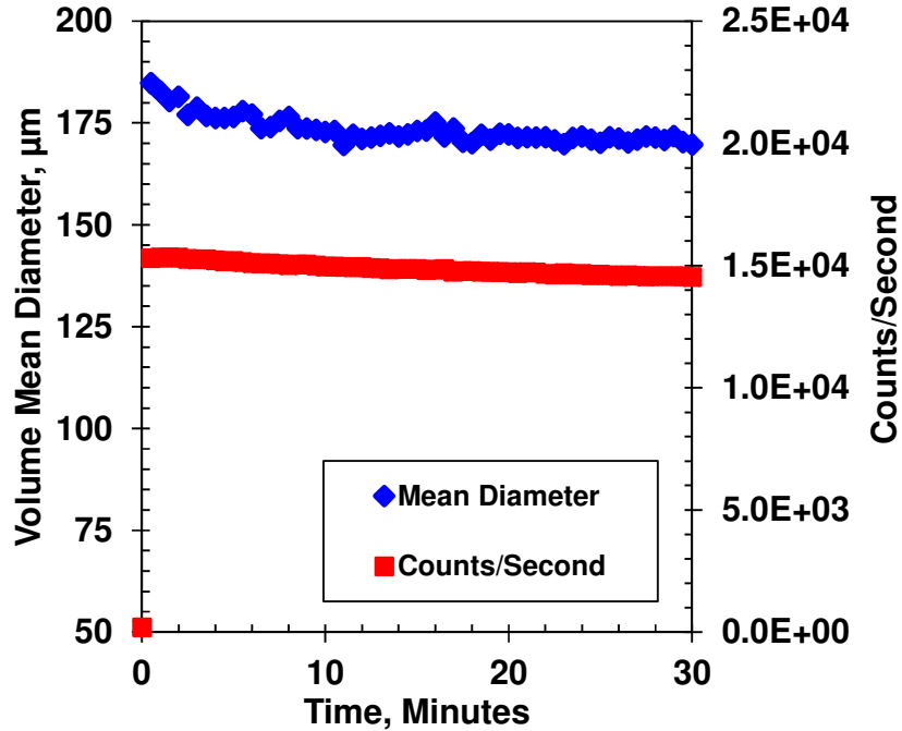
Figure 6.2: Volume mean diameter and number count of asphaltene flocculation over time from 87.5 wt% n -heptane diluted bitumen using the two-stage mixing method at a mixing speed of 195 rpm, and 23°C.
