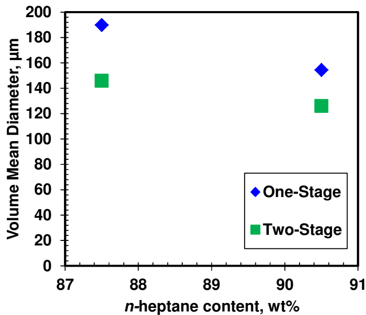
Figure 6.11: Effect of mixing scheme on the steady state volume mean diameter of asphaltene flocs after 30 minutes at 195 rpm and 23°C.
