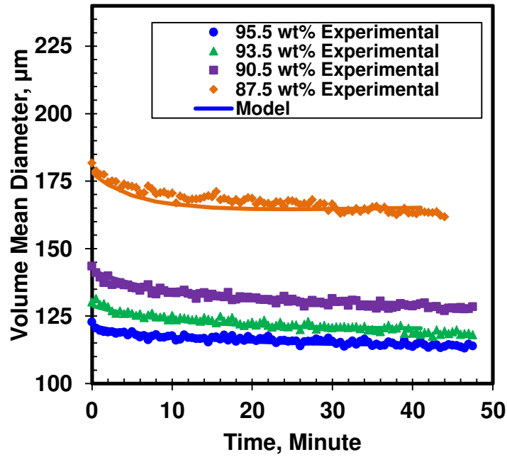
Figure 6.21: Case 2 (constant k_s ) model fitted to data for 87.5 to 95.5 wt% n -heptane diluted bitumen using the two-stage mixing method and a mixing speed of 195 rpm at 23°C.
