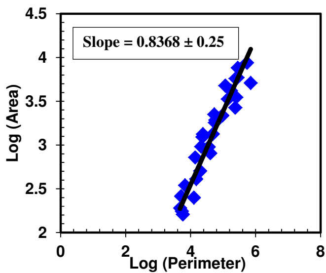
Figure 6.15: Determination of perimeter-based asphaltene aggregates fractal dimension from image analysis of flocs from 87.5 wt% n -heptane in bitumen at 23°C.
