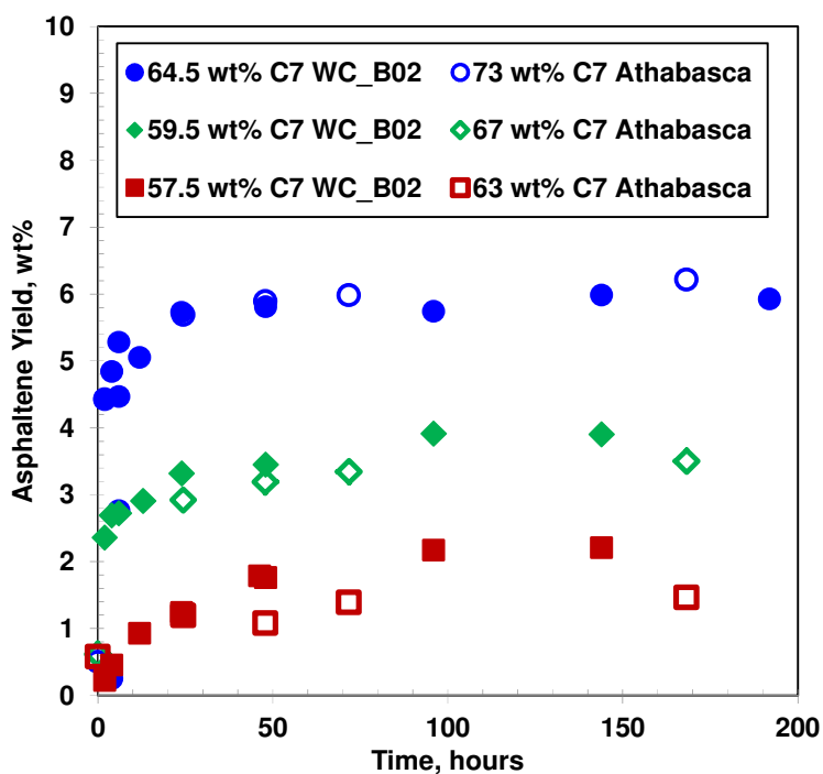
Figure 4.7: Comparison of asphaltene kinetics from WC_B2 bitumen (Shafiee, 2014) and Athabasca bitumen (Beck et al. , 2005) both diluted with n -heptane in Nitrogen at 23°C and 1 atm. Error bars in yield of \pm 0.61 wt% (Shafiee, 2014), and \pm 0.75 wt% (Beck et al. , 2005) are not shown to avoid clutter.
