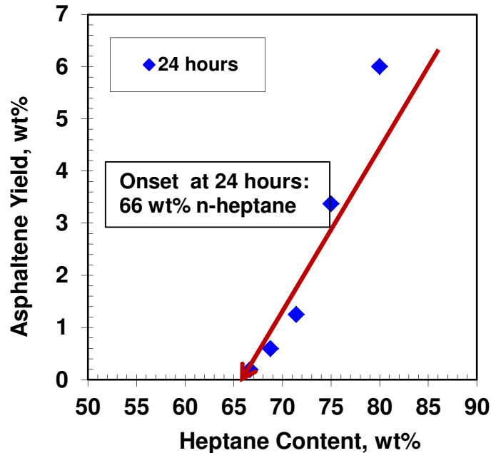
Figure 2.3: The gravimetrically determined onset and yield of asphaltene precipitation from n -heptane diluted with Athabasca bitumen at 24 hours at 23°C (adapted from Beck et al. , 2005).
