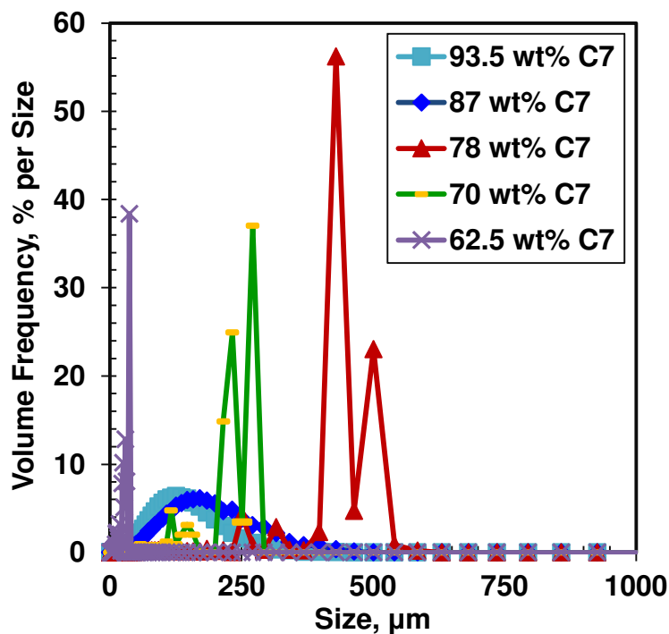
Figure 6.4: Measured volume frequency distribution for low and high n -heptane (C7) diluted bitumen after 60 minutes using two-stage mixing method at 195 rpm, and 23°C.
