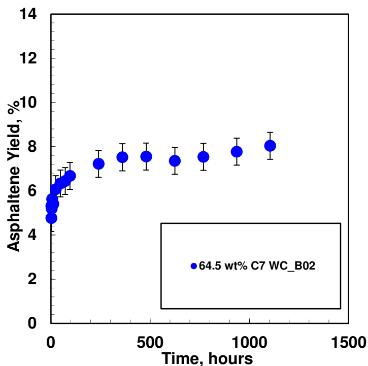
Figure 4.9: Asphaltene precipitation over longer run from WC_B2 bitumen diluted with n -heptane in air at 23°C and 1 atm.
