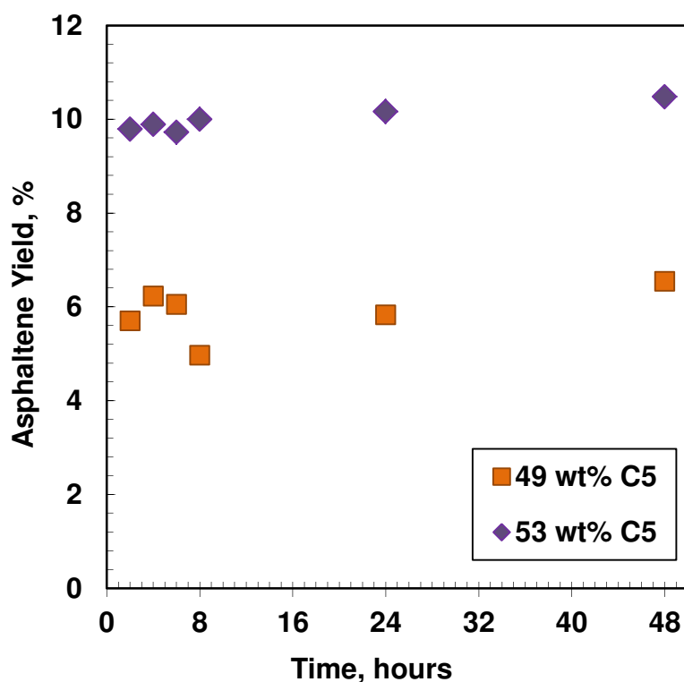
Figure 4.13: Asphaltene precipitation from WC_B_B03 bitumen (Motahhari, 2013) diluted with n -pentane in air at 23°C and 1 atm.
