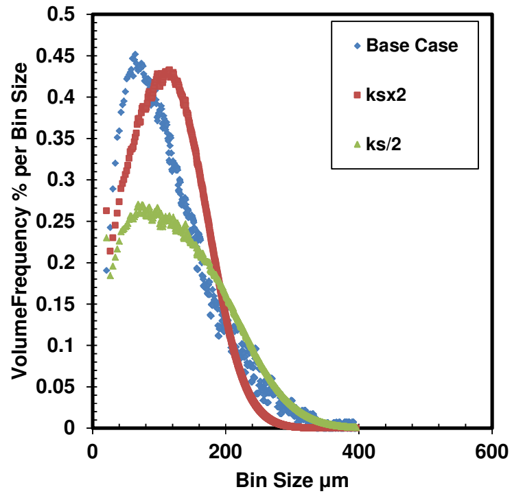
Figure 6.32: Effect of adjusting a) k_s and b) \beta on the volume frequency distribution.
