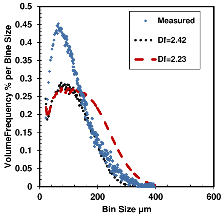
Figure 6.29: Effect of adjusting D_f on the volume frequency distribution for 87.5 wt% n -heptane diluted bitumen using the two-stage mixing method and a mixing speed of 195 rpm at 23°C.
