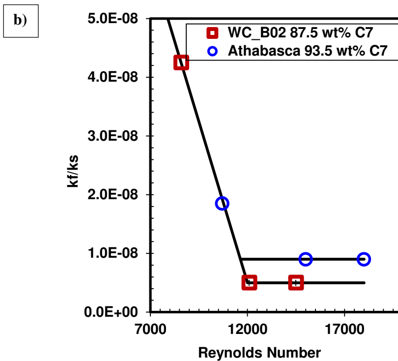
Figure 6.30: Summary of k_f/k_s ratio for a) 87.5-95.5 wt% at 195 rpm and 87.5 wt% at different shear, b) comparison of two bitumens, WC_B02 and Athabasca.
