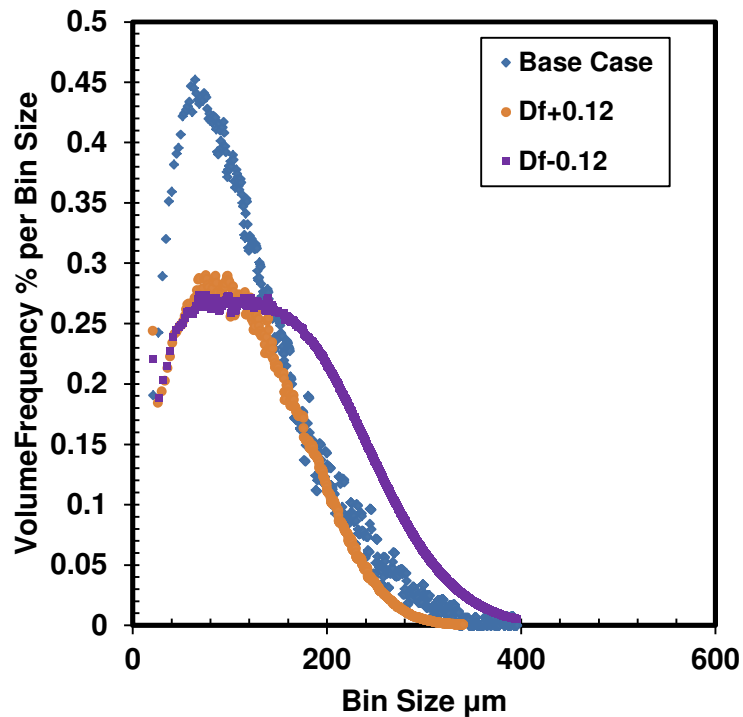
Figure 6.37: Effect of adjusting D_f on the volume frequency distribution.
