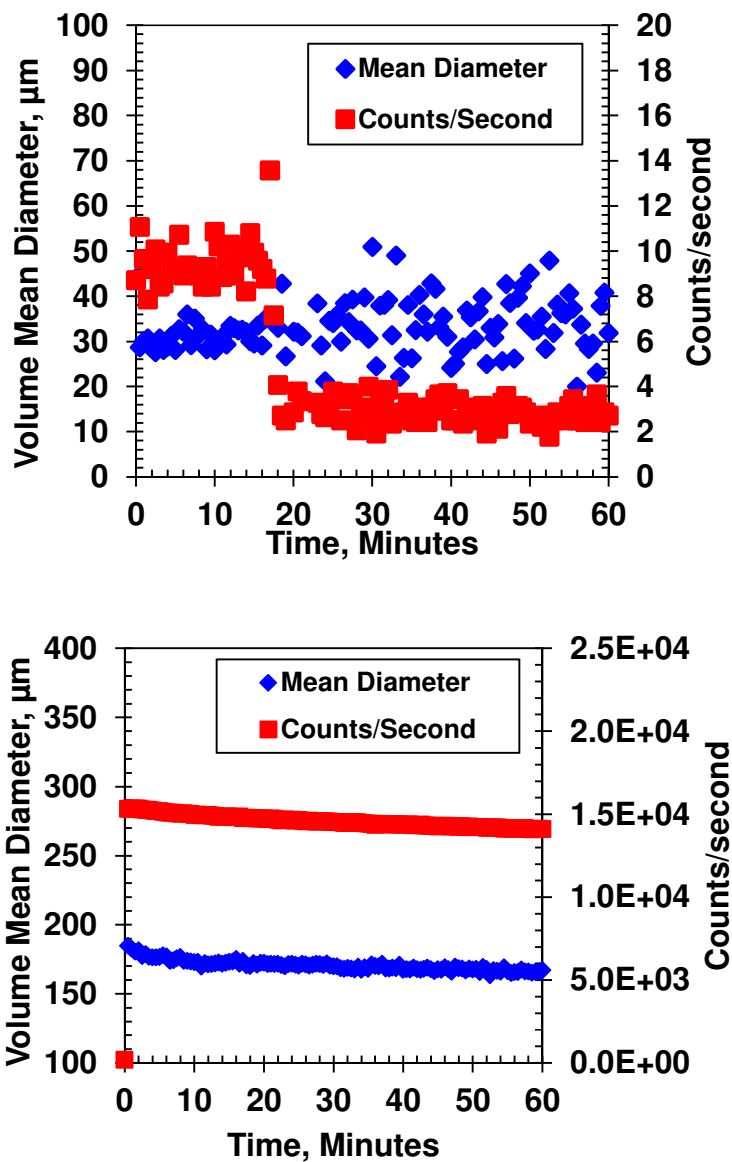
Figure 3.4: Measured volume mean diameter and particle count distribution for a) low dilution of 62 wt%, and b) high dilution of 87.5 wt% n -heptane, at 195 rpm and 23°C.
