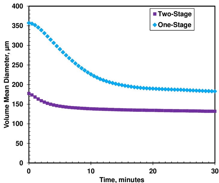
Figure 6.12: Effects of mixing scheme on the kinetics of asphaltene flocculation for 90.5 wt% n -heptane, at 195 rpm and 23°C.
