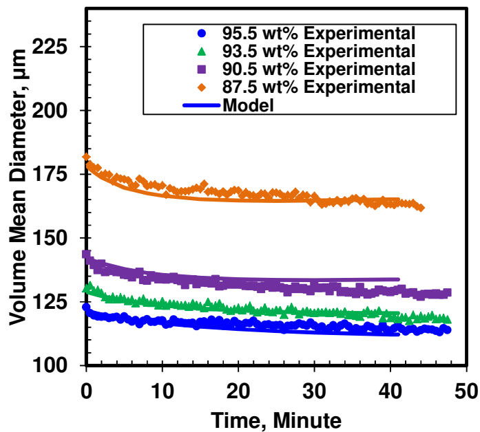
Figure 6.24: Case 4 (correlated k_f/k_s ratio and constant k_s ) model results for 87.5 to 95.5 wt% n -heptane diluted bitumen using the two-stage mixing method and mixing speed of 195 rpm at 23°C.
