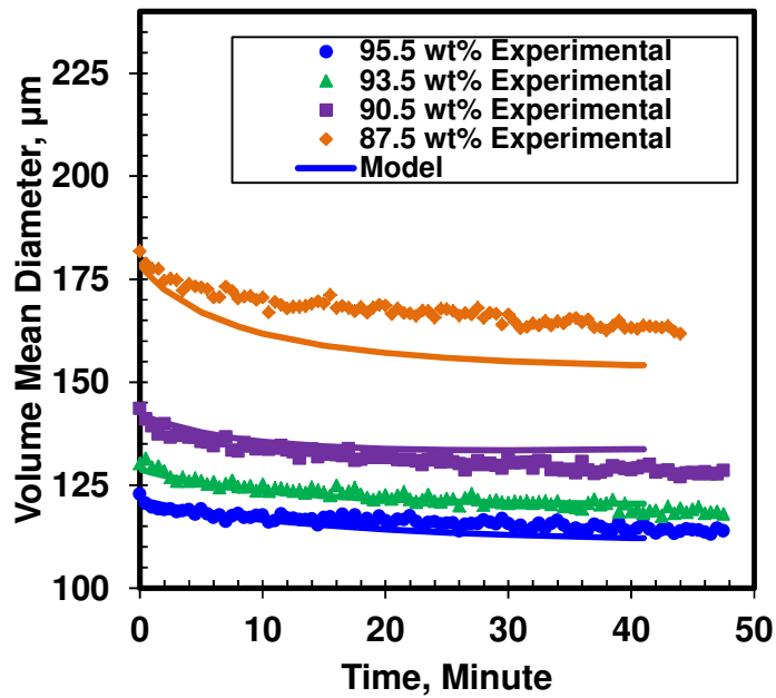
Figure 6.23: Case 3 (constant k_f/k_s ratio and k_s ) model results for 87.5 to 95.5 wt% n -heptane diluted bitumen using the two-stage mixing method and mixing speed of 195 rpm at 23°C.
